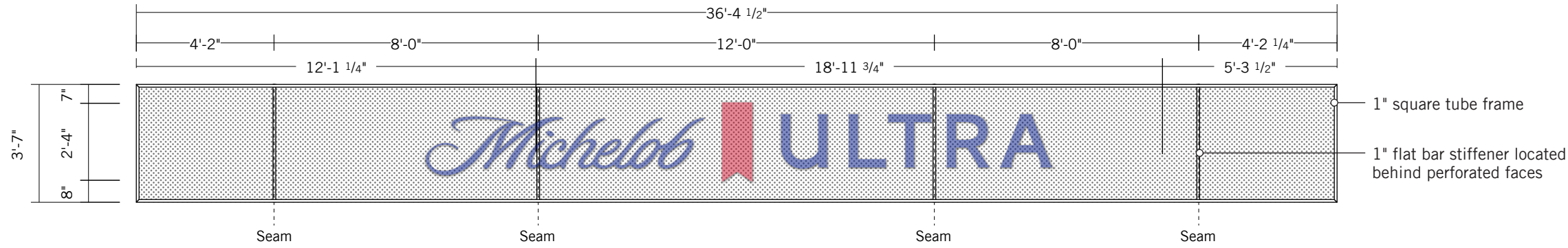
FRAME VIEW
