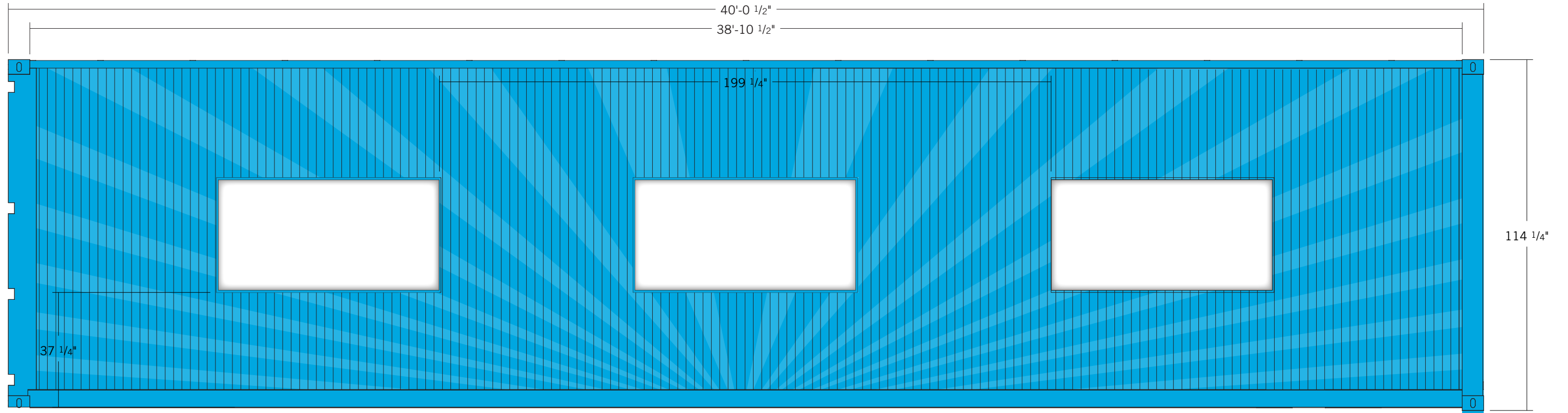
EX.01.1 - CONTAINER SUNBURST PAINTMASK - BOTH FRONT AND BACK
