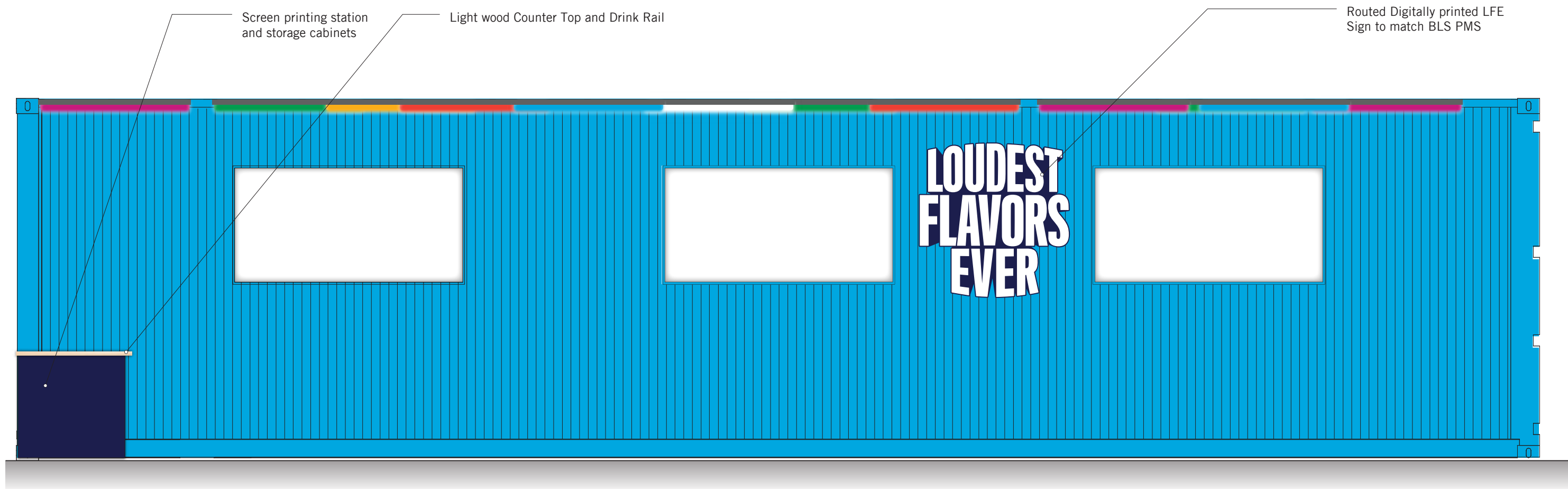
IN.02 - ELEVATION - RIGHT SIDE
