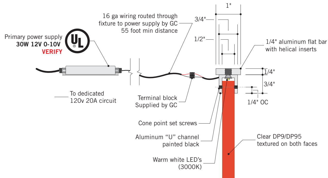
IN.01 - ACRYLIC LIGHTING FEATURES - SIDE VIEW - PREFERRED OPTION
