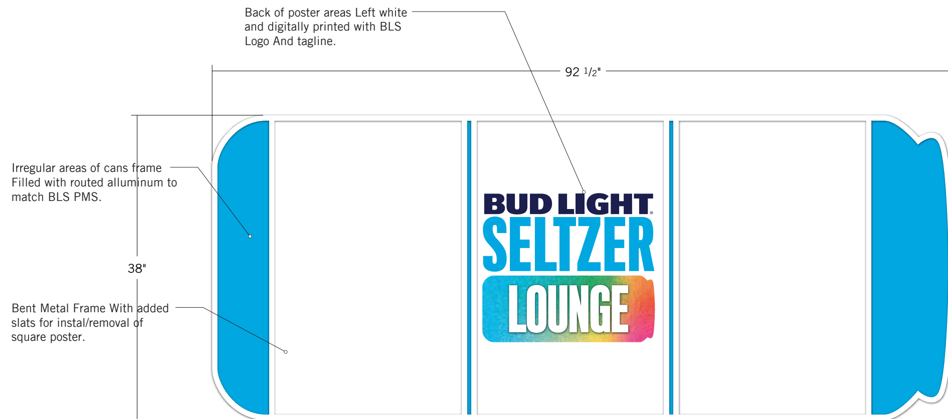
DETAIL - BLS CAN POSTER FRAME
